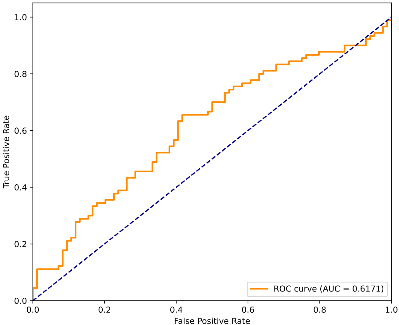
ROC Curve - GaussianNB
